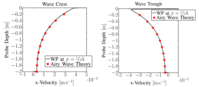
Fig. 7. Velocity profiles for increasing depth beneath wave troughs and crests, calculated from Airy wave theory and measured 1/2\lambda from the wave maker
