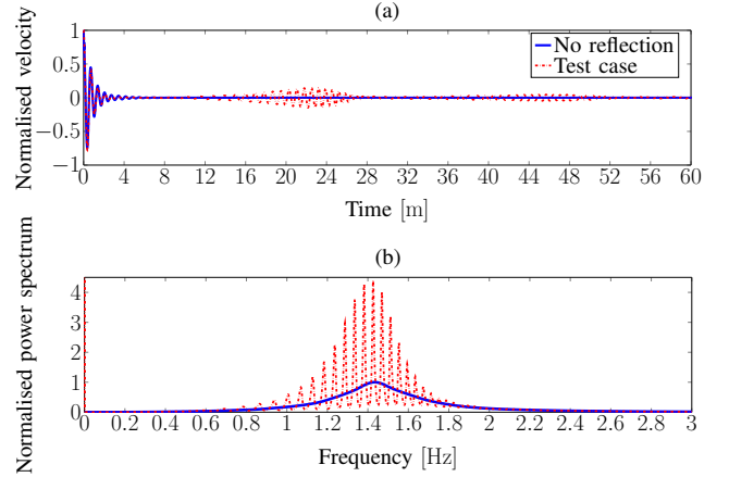
Fig. 17. (a) Time series of the WEC velocity in free decay experiment (b) The power spectrum of the time series
