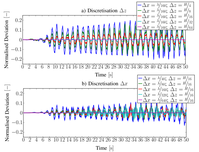
Fig. 3. Mesh convergence study: Deviation of FSE (normalised by wave amplitude), for different mesh resolutions, compared to the finest mesh case
